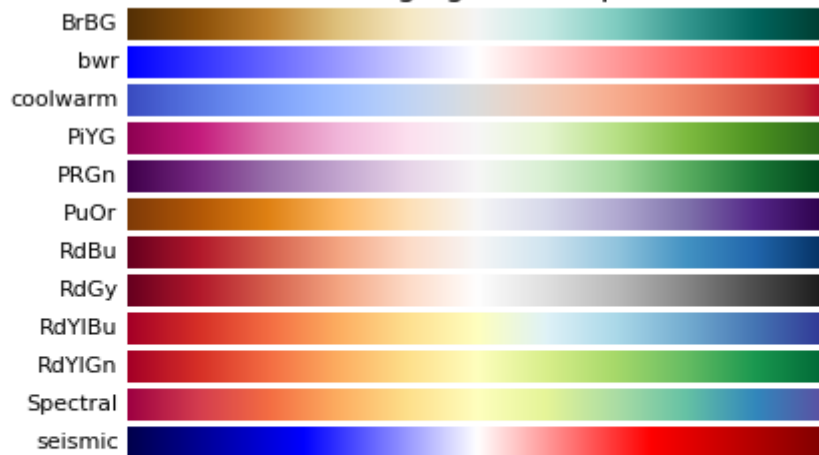
Diverging colormaps
