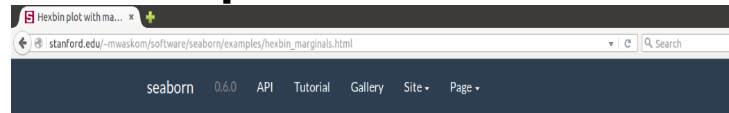
Hexbin plot with marginal distributions
